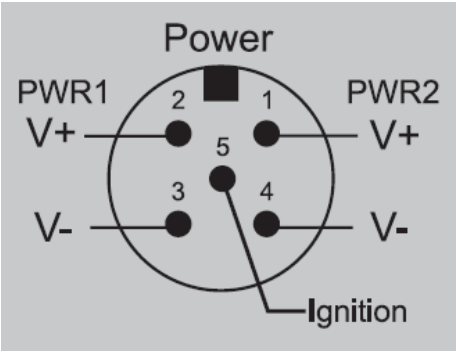
Pin assignment of Power input
