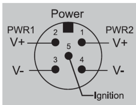
Pin assignment of Power input (IGN models)
