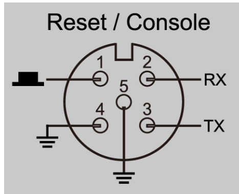
Pin assignment of reset function
