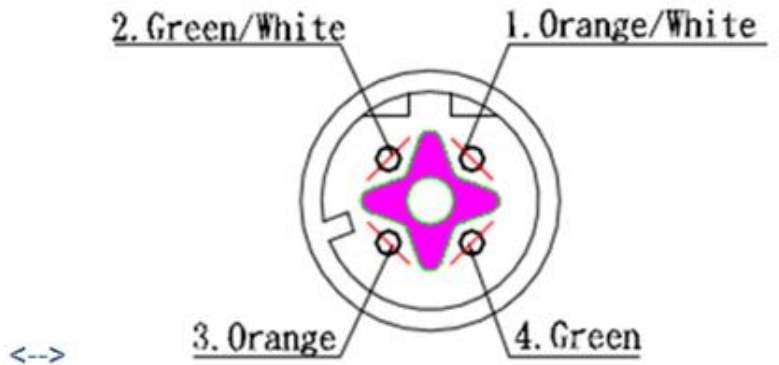
Cable connector
