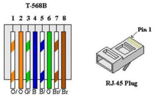
Cable connector
