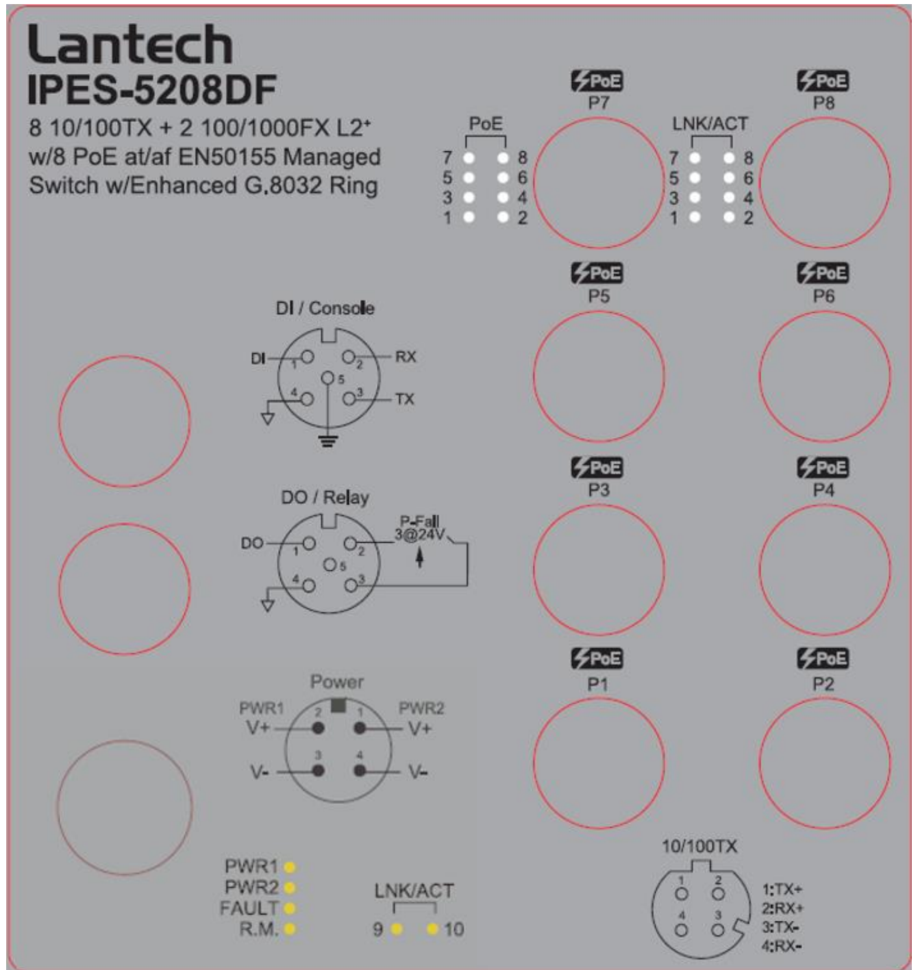
Front panel of IPES-5208DF
