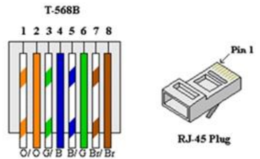
Cable connector
