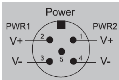
Pin assignment of Power input (Shipping after May 2018)
