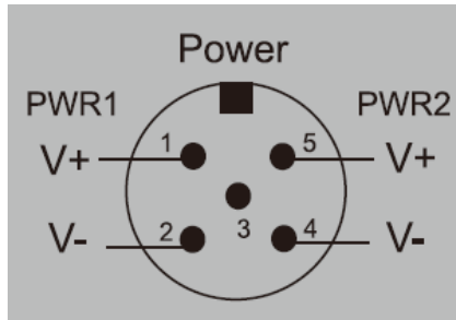
Pin assignment of Power input (Shipping before Q1 2018)
