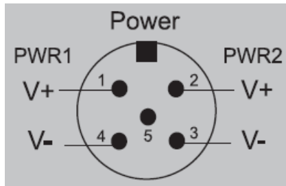
Pin assignment of Power input (Shipping after Jan 2018)
