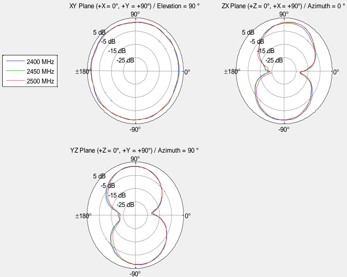
C65-P205 2G Band = 2400 - 2500 MHz % 2G Band
