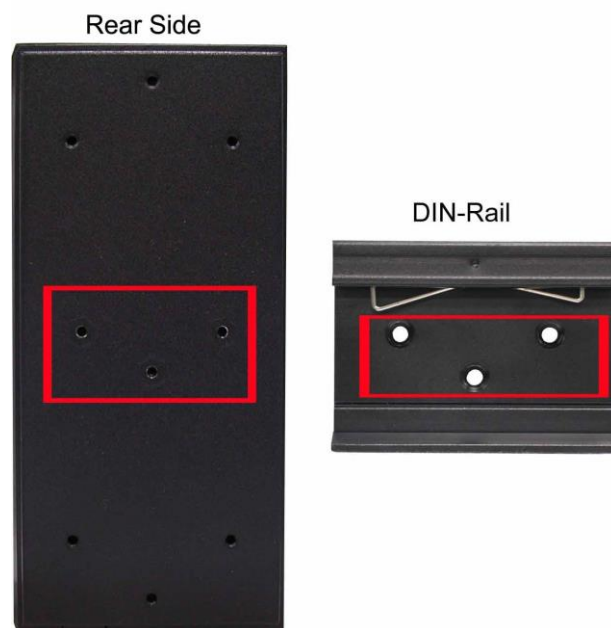
Figure-10: Rear side of the PoE Injectors Industrial Switch
