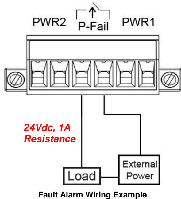
Terminal Block Plugs for Fault Alarm Contacts
