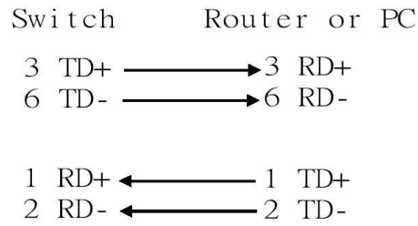
Straight Through Cable Schema
