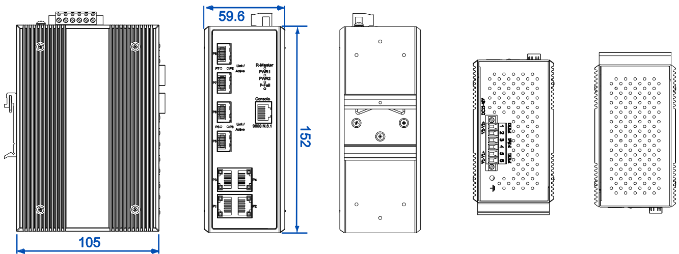
Mechanical Dimensions
