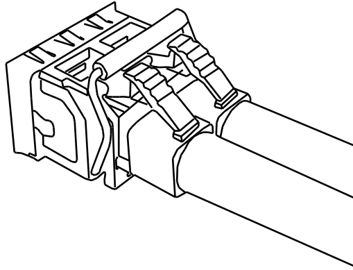
LC connector to the transceiver
